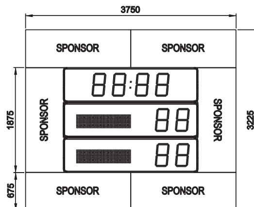
BT 2045 Alpha + Peripheral advertising panels
